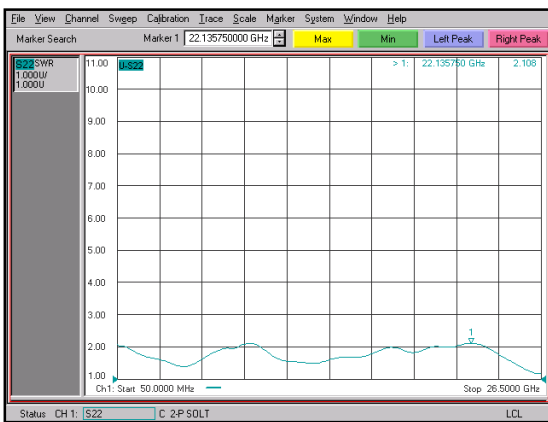
Insertion Loss
