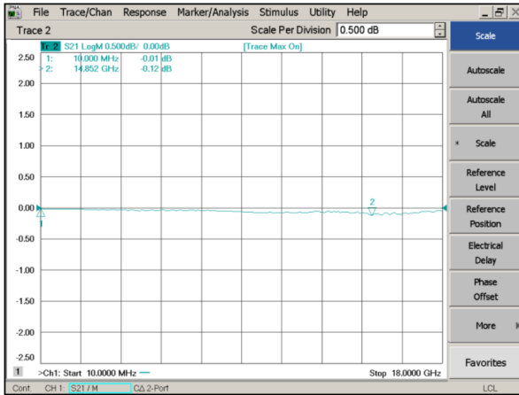
Amplitude Balance
