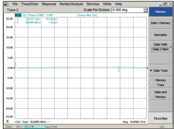
Phase Balance
