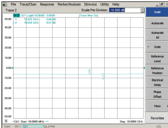
Insertion Loss
