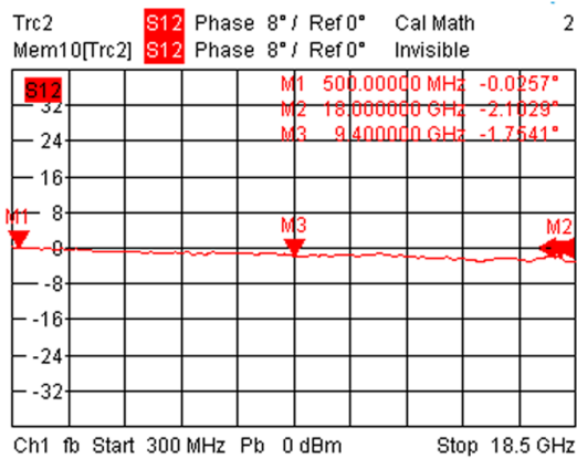
Phase Unbalance
