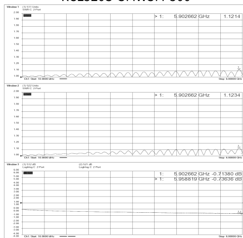
RCE520S-SMWSM-500
