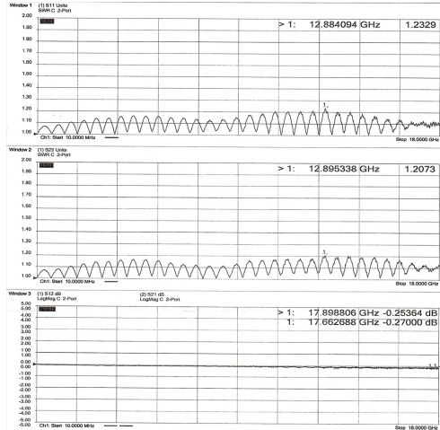
RCA510-SMSM-1M
