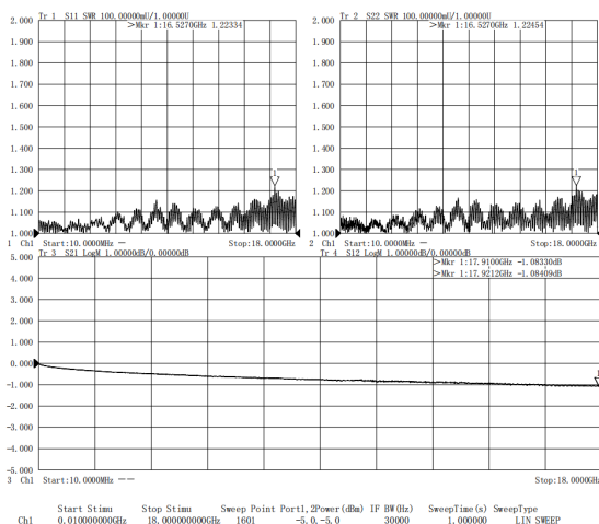
RCA510-SMSM-1M
