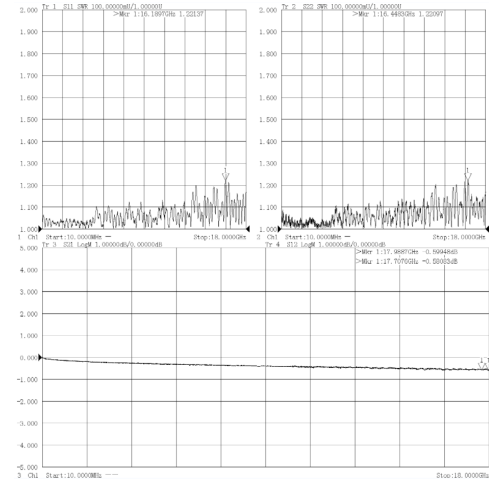
RCA510-SMSM-2M
