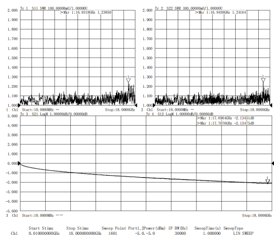
RCA510-SMSM-2M
