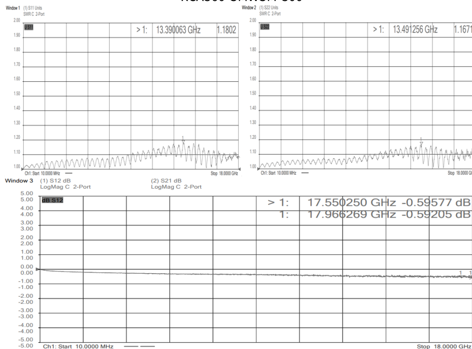
RCA360-SMWSM-300
