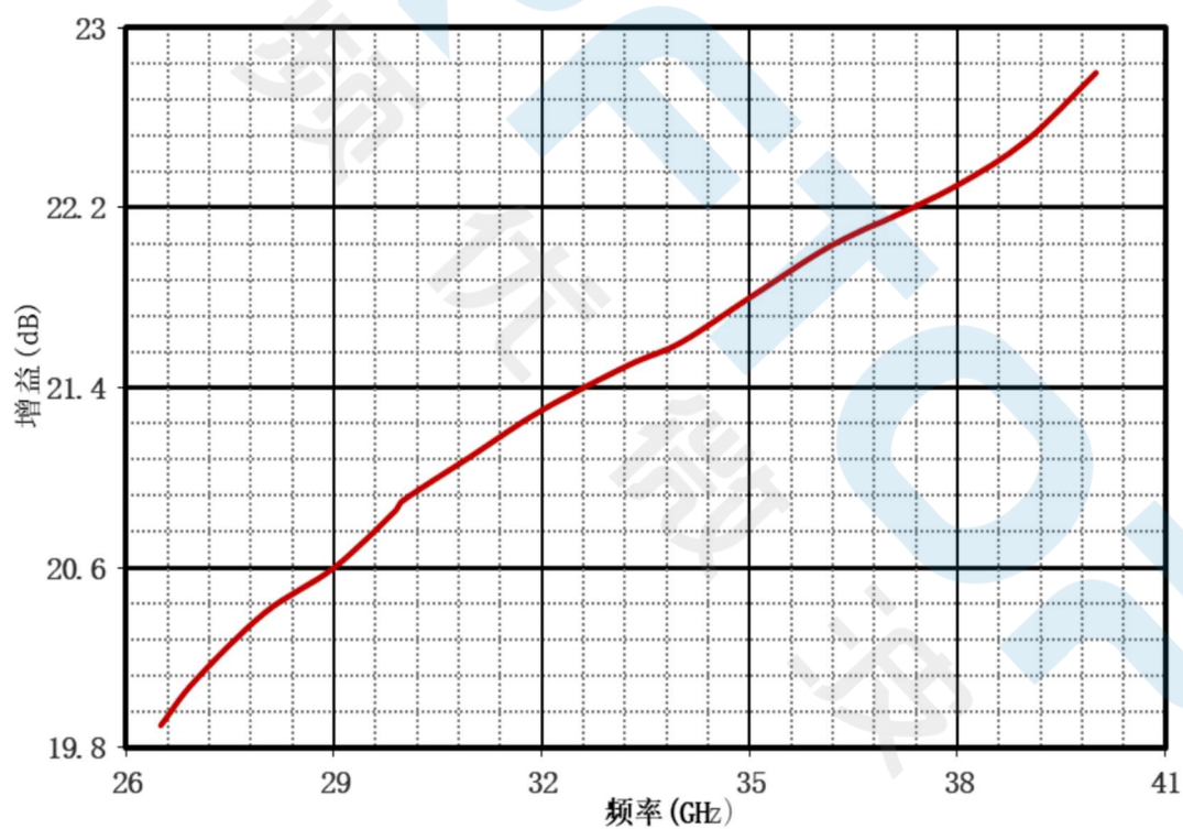
Frequency vs Gain
