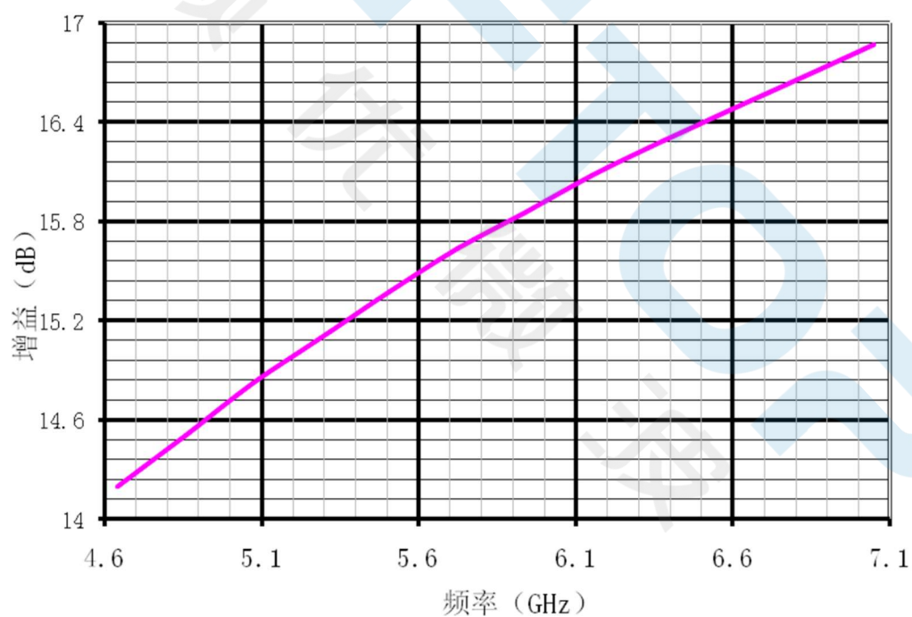
Frequency vs Gain
