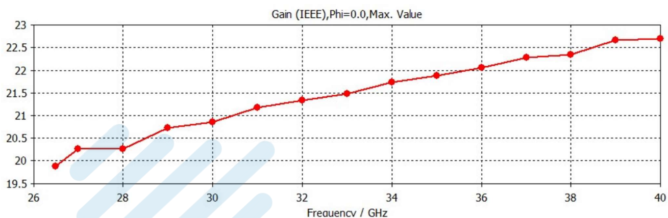
Frequency vs Gain
