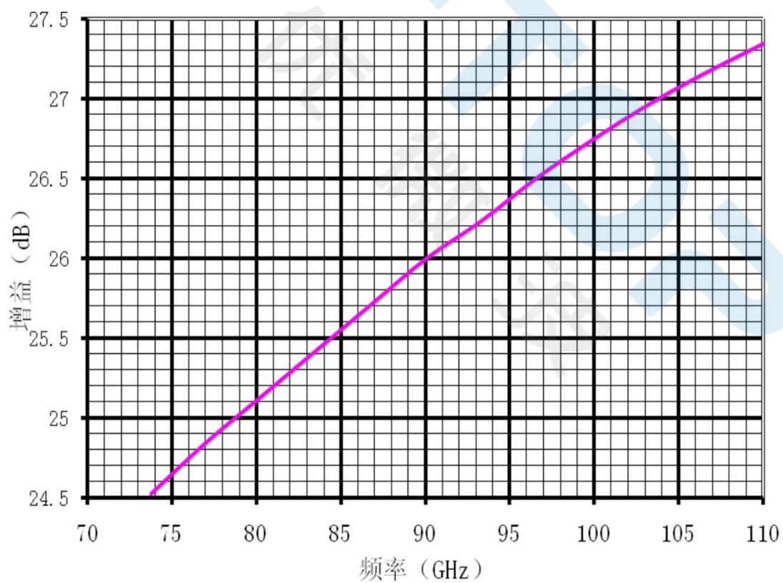
Frequency vs Gain
